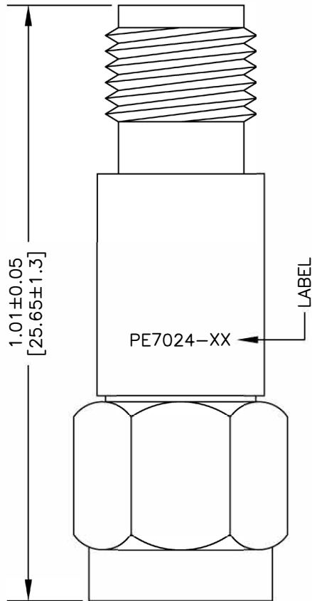
SMA MALE
