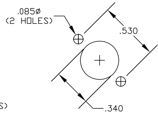
MOUNTING HOLES
