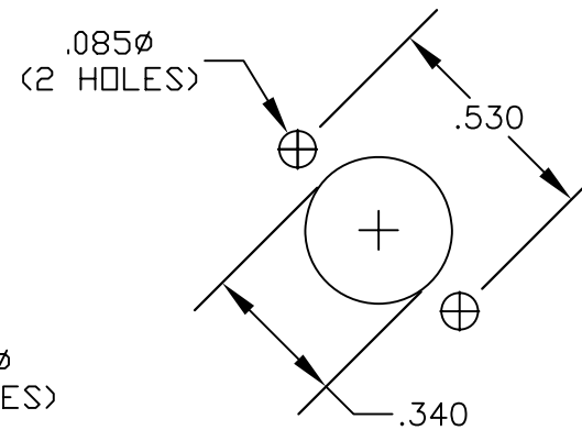
MOUNTING HOLES
