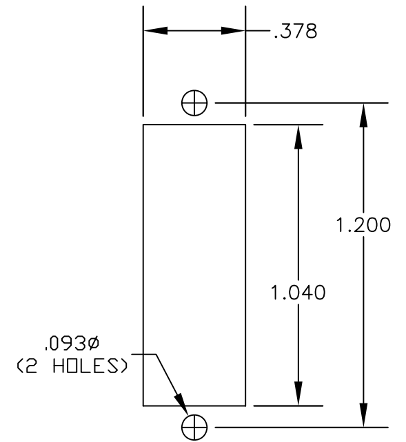
MOUNTING HOLES
