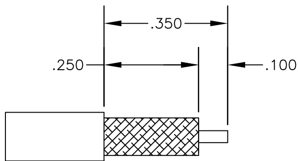
STRIPPING DIMENSIONS
