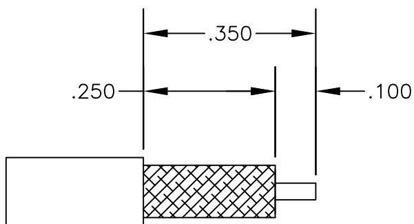
STRIPPING DIMENSIONS
