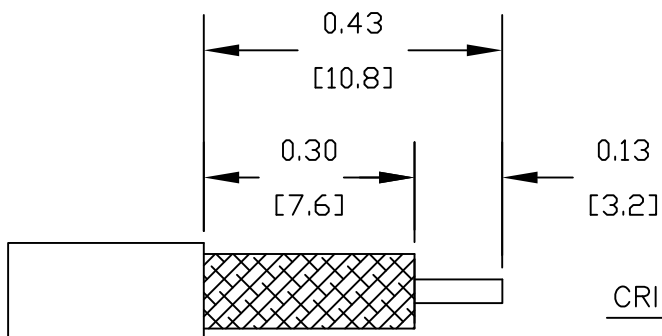
STRIPPING DIMENSIONS
