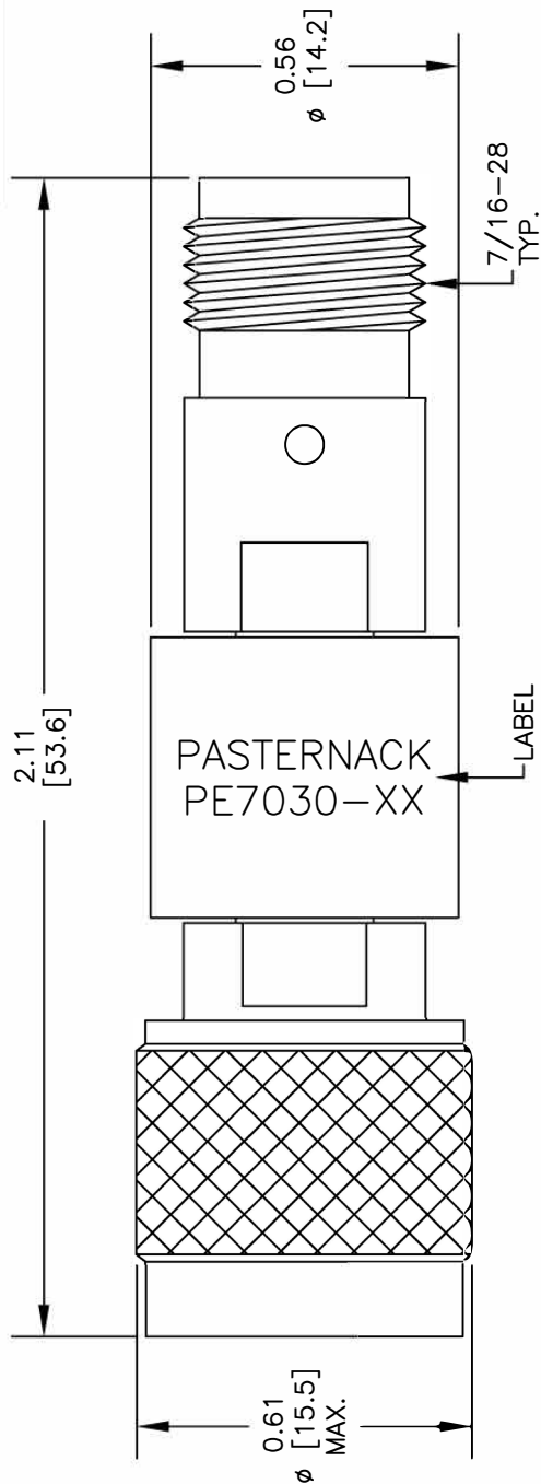
TNC FEMALE
