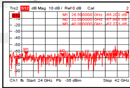
Isolation @+25°C
