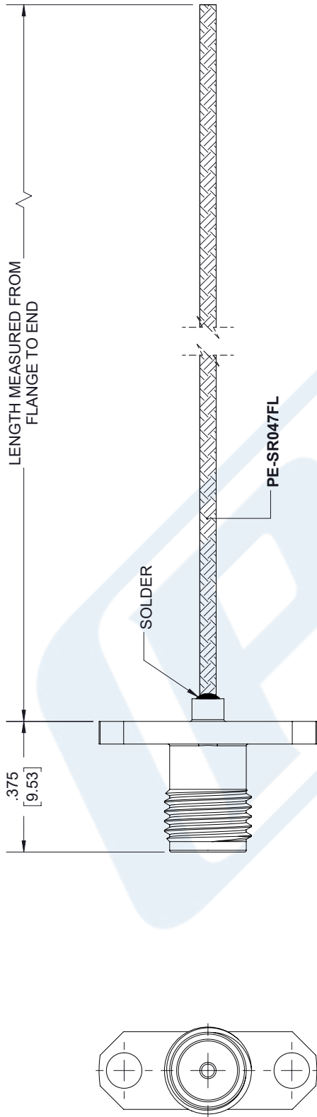
SMA FEMALE 2 HOLE FLANGE
