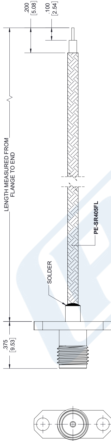
SMA FEMALE 2 HOLE FLANGE
