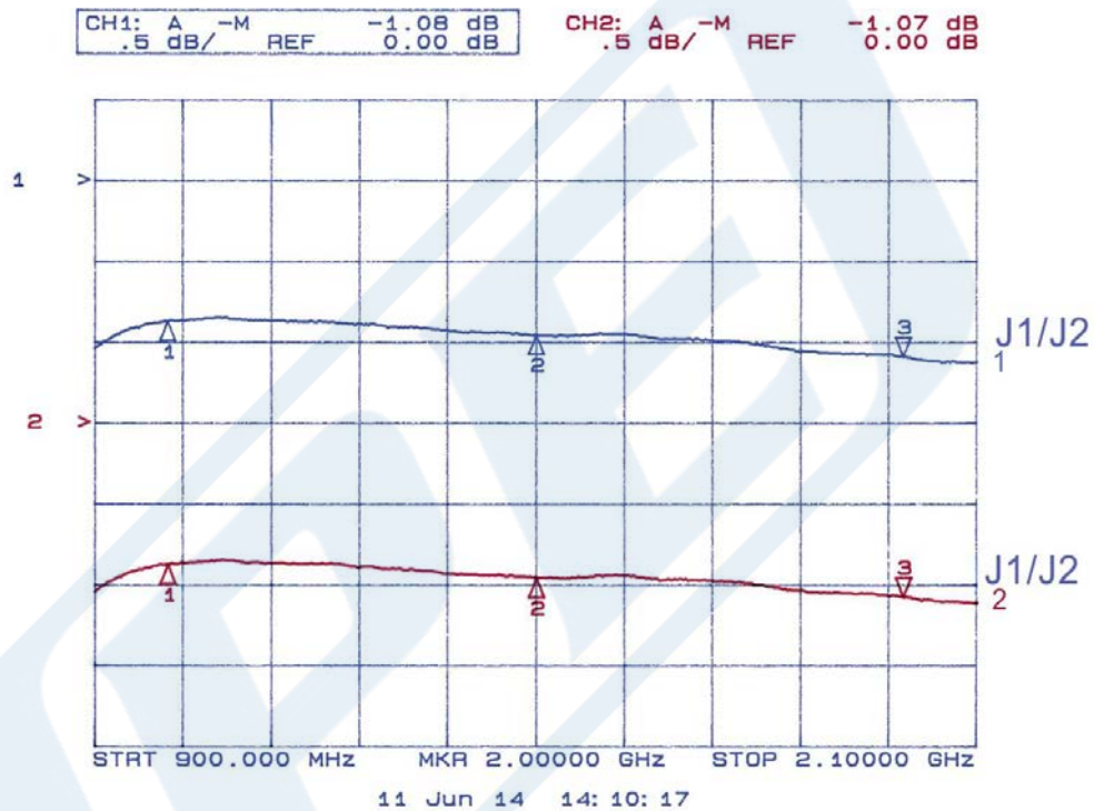
Insertion Loss
