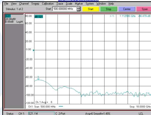
(J1 – J3) Isolation
