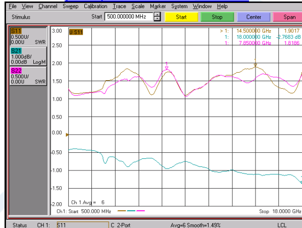
(J1 – J4) Insertion Loss and Return Loss
