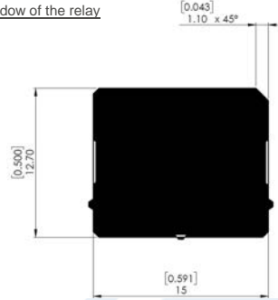
Video shadow of the relay
