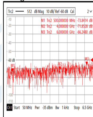
Isolation@-40°C
