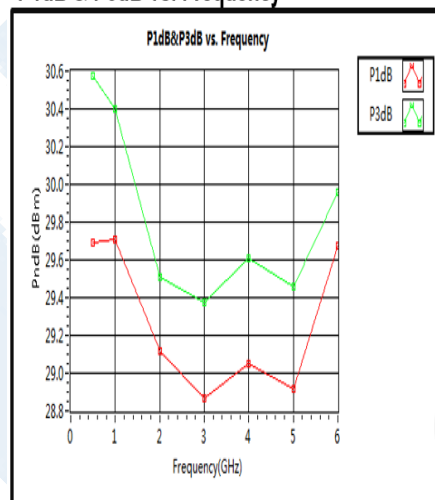
P1dB & P3dB vs. Frequency
