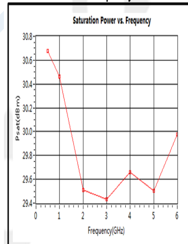
Saturated Power vs. Frequency
