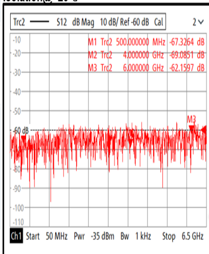
Isolation@+25°C
