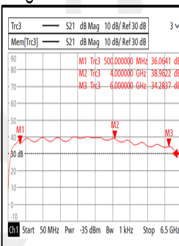
Gain@-40°C
