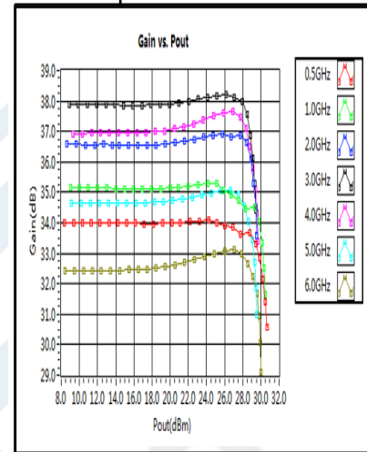
Gain vs. Output Power
