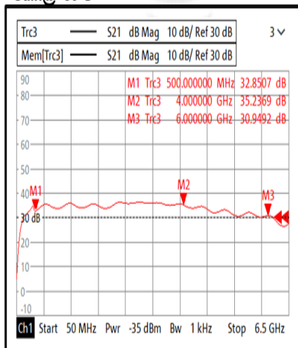
Gain@+85°C
