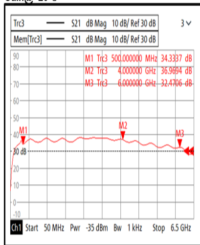
Gain@+25°C
