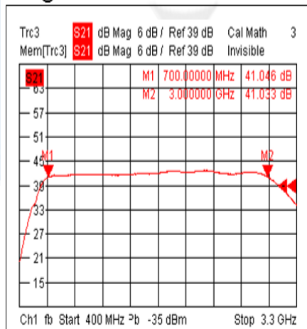
Gain@+70°C
