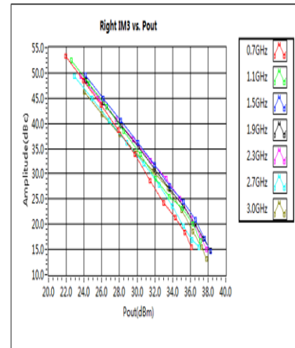
Right IM3 vs. Pout
