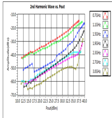
2nd Harmonic Wave Output Power
