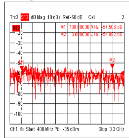
Isolation@-40°C
