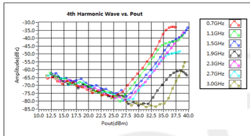
4th Harmonic Wave Output Power
