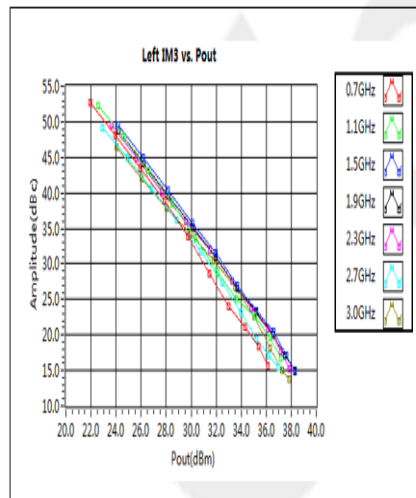
Left IM3 vs. Pout
