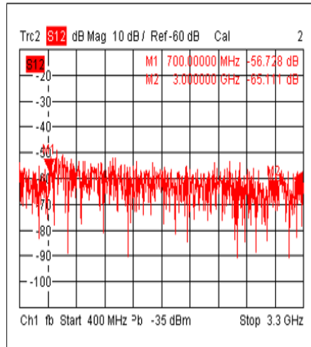
Isolation@+70°C
