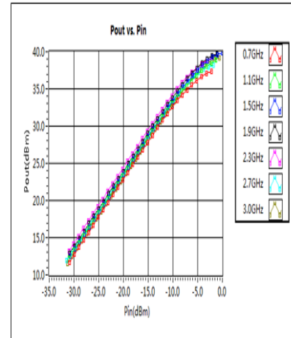
Pout vs. Pin
