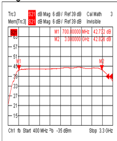
Gain@+25°C
