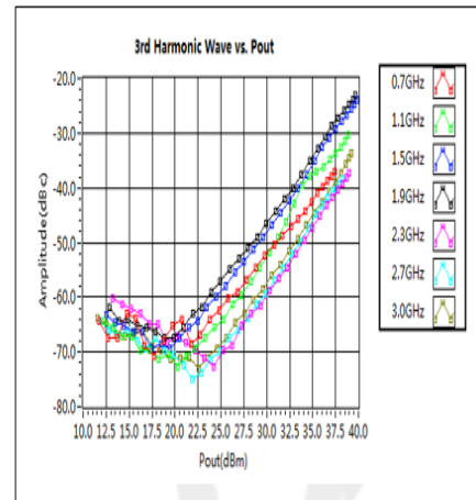
3rd Harmonic Wave Output Power
