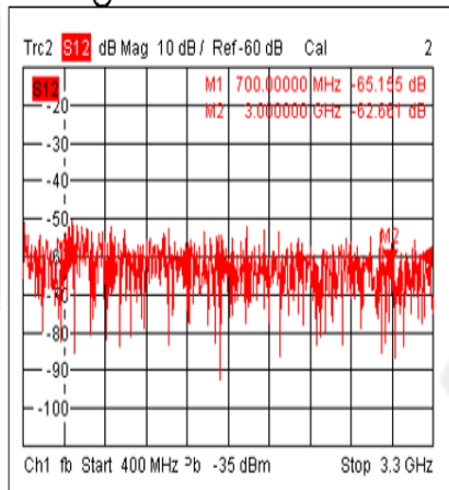
Isolation@+25°C
