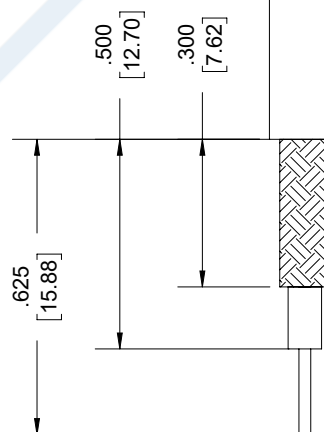
STRIPPING DIMENSIONS
