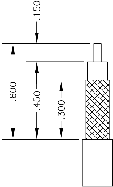
CRIMP SIZES REQUIRED
