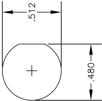
MOUNTING HOLE
