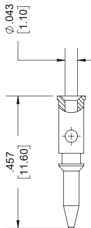
CONTACT
