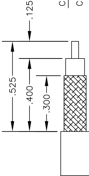
STRIPPING DIMENSIONS
