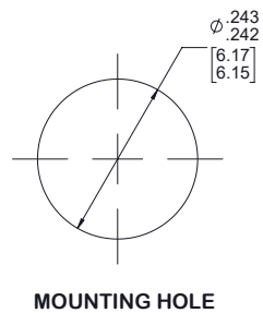
MOUNTING HOLE
