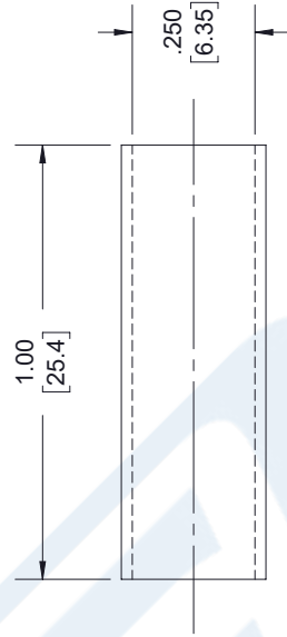
SHRINK TUBE
