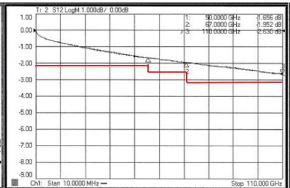
S12 Insertion Loss, dB
