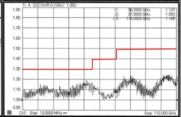
S22 VSWR
