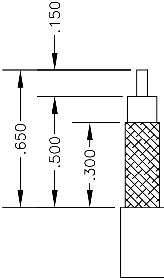
STRIPPING DIMENSIONS
