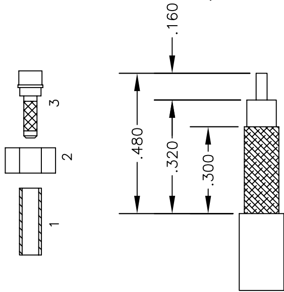
STRIPPING DIMENSIONS
