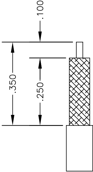
STRIPPING DIMENSIONS
