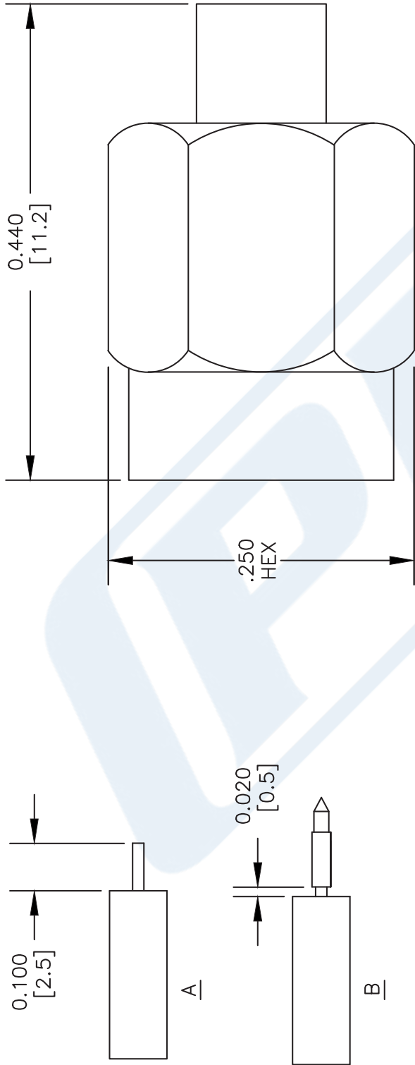
STRIPPING DIMENSIONS
