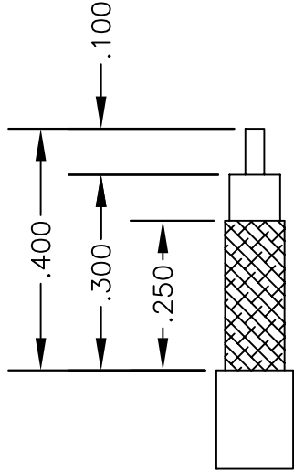
STRIPPING DIMENSIONS
