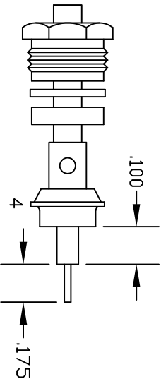
ASSEMBLY (B)
