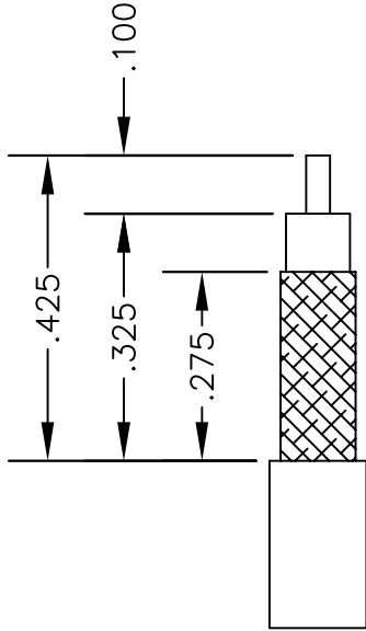
STRIPPING DIMENSIONS
