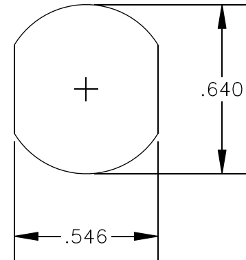
MOUNTING HOLE
