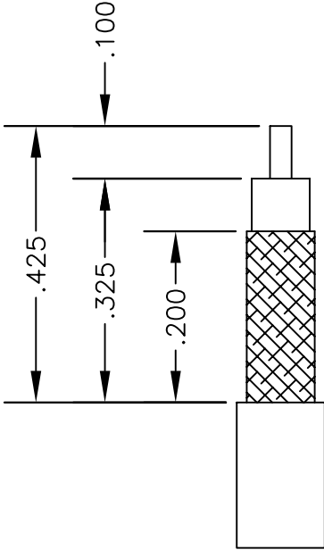
STRIPPING DIMENSIONS
