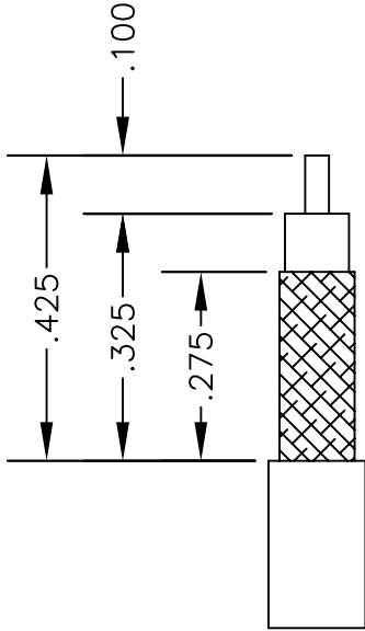
STRIPPING DIMENSIONS
