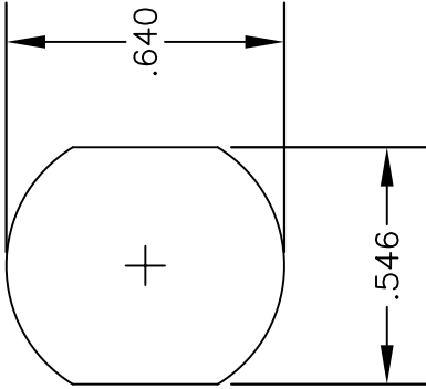
MOUNTING HOLE
