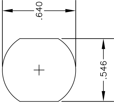
MOUNTING HOLE
