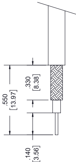
STRIPPING DIMENSIONS
