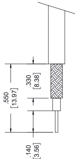
STRIPPING DIMENSIONS
