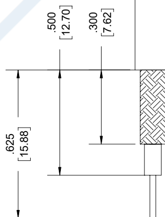
STRIPPING DIMENSIONS
