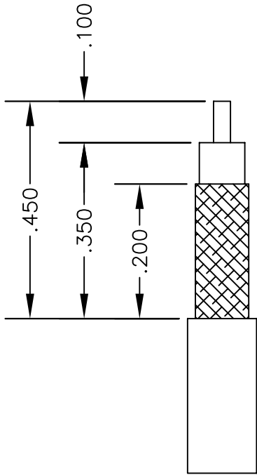
STRIPPING DIMENSIONS
