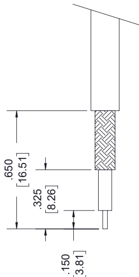
STRIPPING DIMENSIONS
