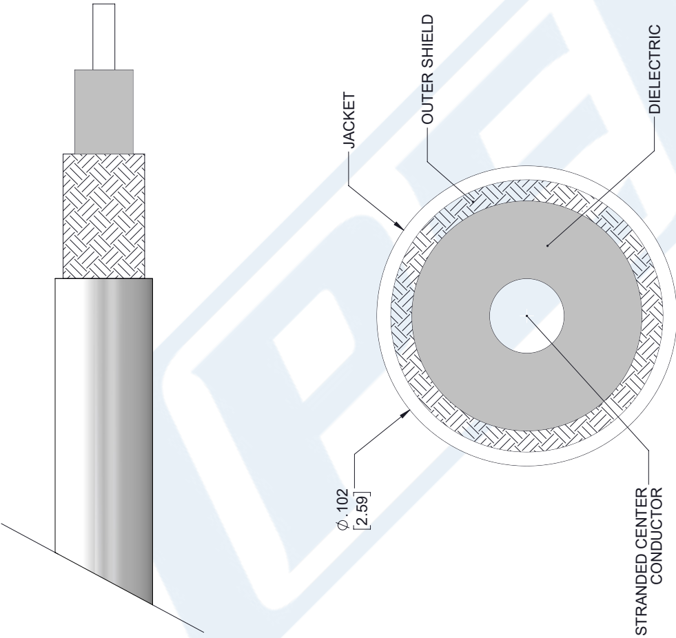
SECTION VIEW
