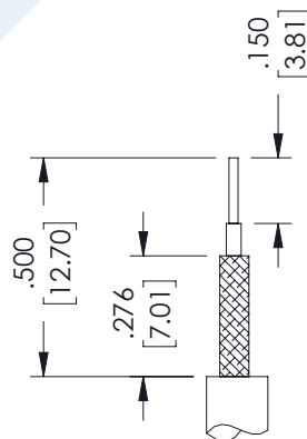
STRIPPING DIMENSIONS
