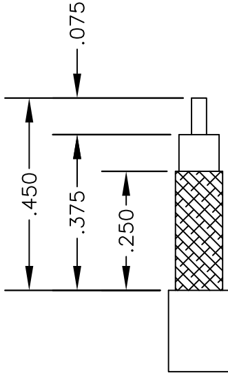
STRIPPING DIMENSIONS
