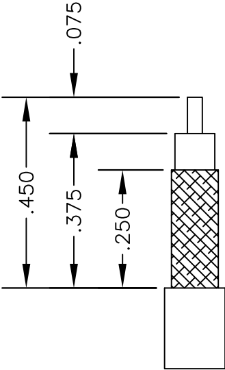
STRIPPING DIMENSIONS
