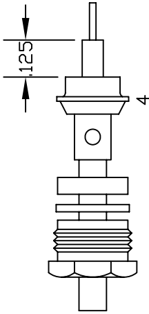
ASSEMBLY (B)
