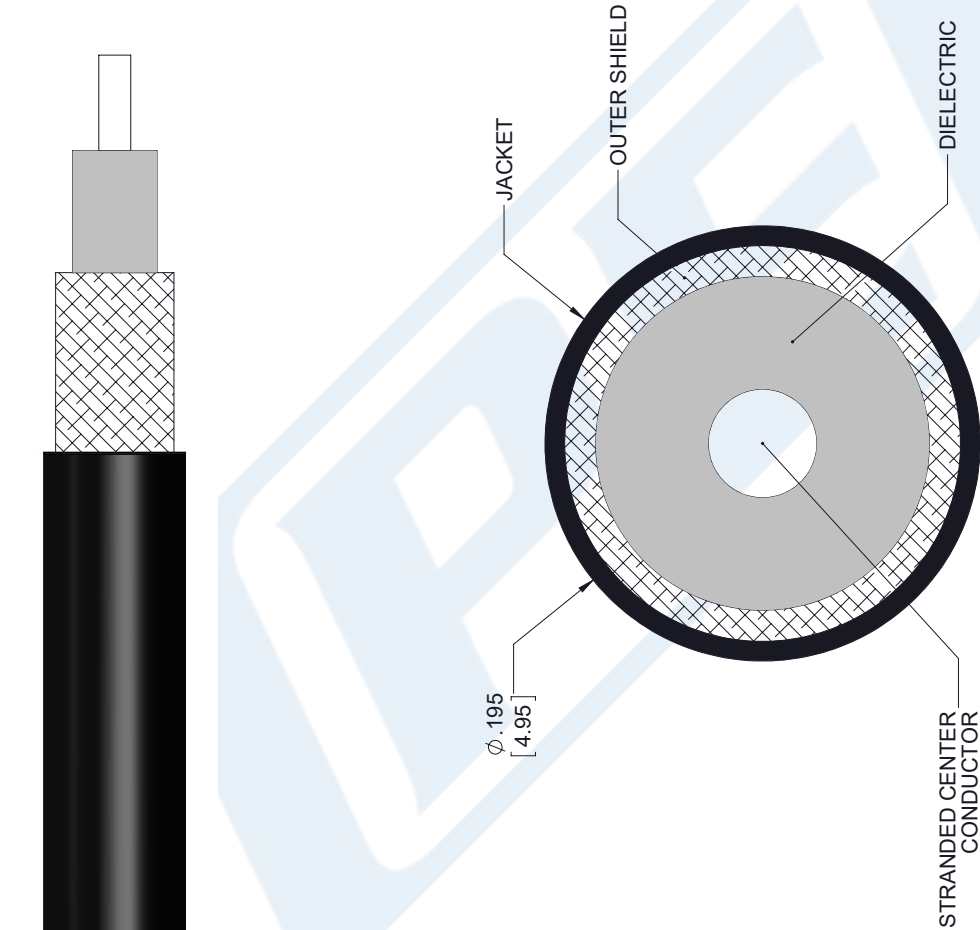
SECTION VIEW
