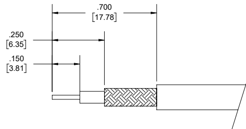
STRIPPING DIMENSIONS
