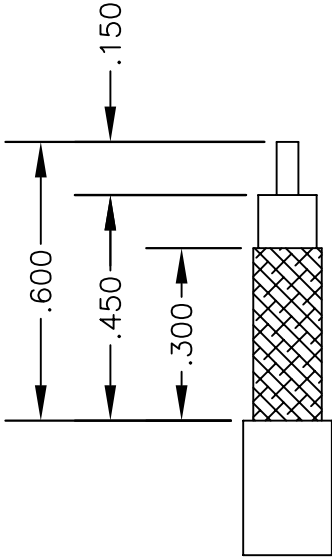
STRIPPING DIMENSIONS
