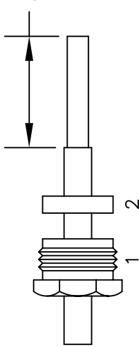
ASSEMBLY (A)
